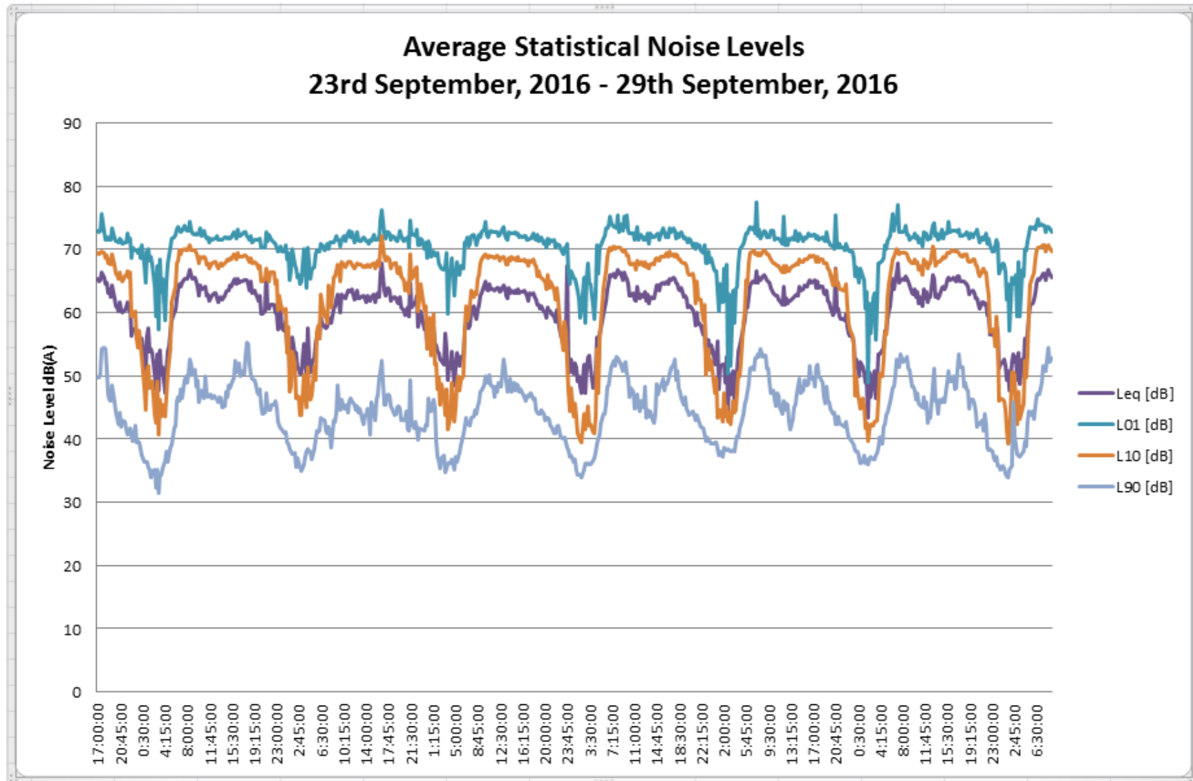
Figure 3 - Noise Survey
